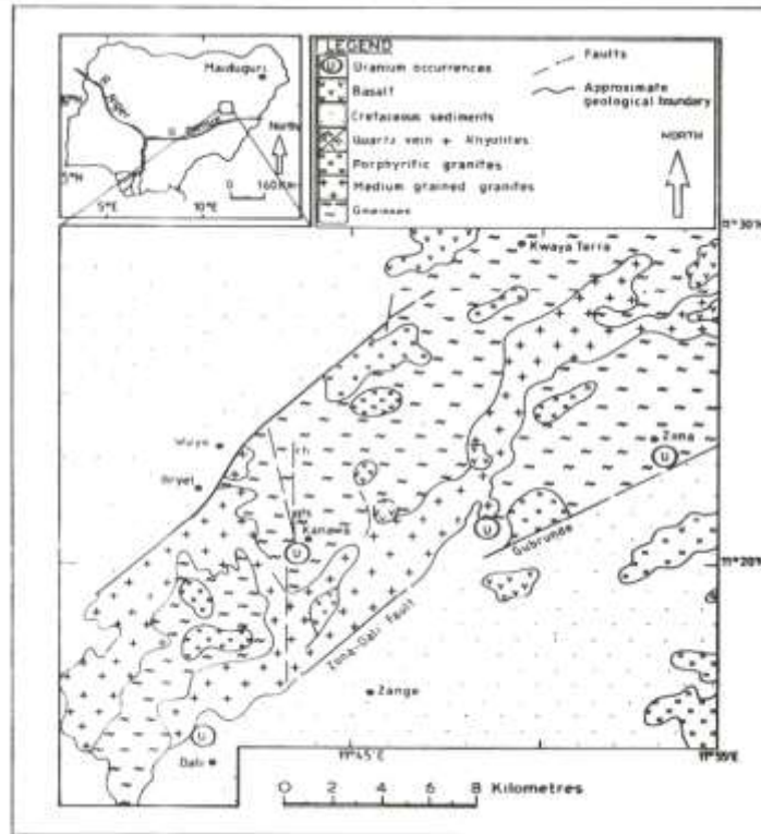
Fig.4. Geologic map of Gubrunde and its environs showing areas of uranium mineralization (After Ige et al,1994: Ige and Funtua, 2000).
